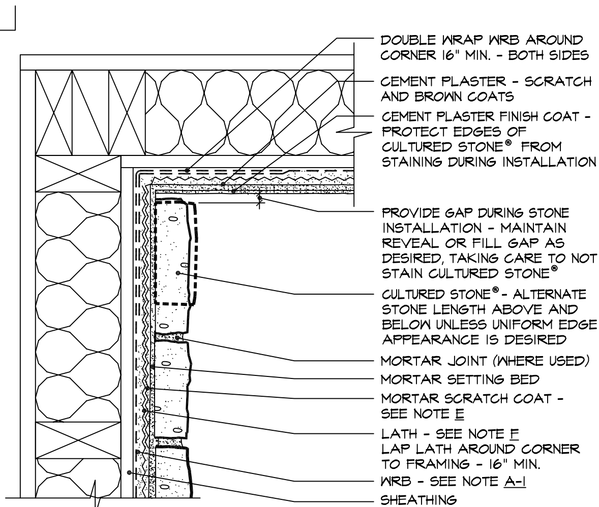
1-B INSIDE CORNER AT CEMENT PLASTER 1.17 SCALE: 3"=1'-0"
